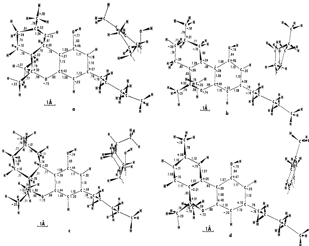
Figure 1. Conformations and charge distributions of (a) \Delta^9 -THC, (b) \Delta^{6a(10a)} -THC, (c) HHC, and (d) cannabimol. The complete structures show the atoms as viewed normal to the plane through C_2 , C_3 , C_4 . The perspectives of the C rings are viewed in the direction parallel to the vector from C_2 to C_{10b} . Net atomic charges are given as signed numbers and overlap populations between atoms as unsigned numbers.
