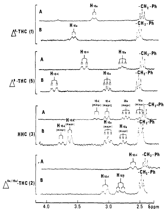
Figure 2. Partial 220-MHz spectra ( \delta 2.5–4.0 region) of 1 , 2 , 3 , and 5 in \text{CDCl}_3 (A) and \text{C}_6\text{D}_6\text{N} (B) solvents.
