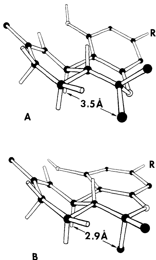
Figure 3. Possible conformations for ring B in \Delta^9 -THC. The internuclear distance between the 6\alpha -methyl and H_{10\alpha} in conformation A was obtained from measurement on Dreiding models; the corresponding distance in conformation B was derived from Westheimer calculations.
